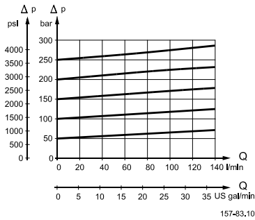
Pressure relief valve characteristic
