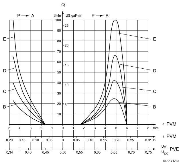
Characteristic of oil flow, spool travel and voltage
