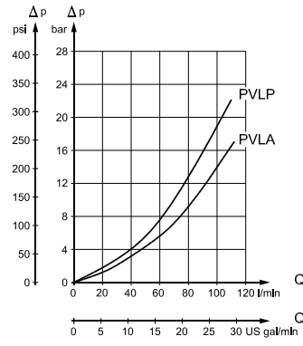
PVLA, suction valve characteristic
