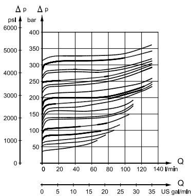
PVLP, shock valve characteristic
