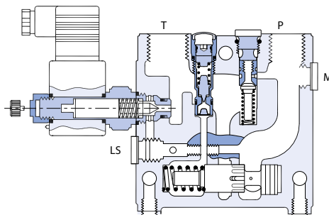
PVPX, electrical LS unloading valve
